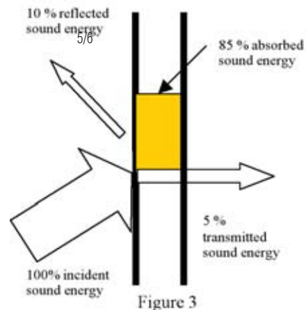
A wall partition designed for high absorption and low reflected and transmitted sound energy.
